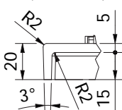
DETAIL X (1 : 2)
